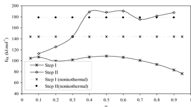
Fig. 7. Dependence of the activation energy on extent of sodium perborate tetrahydrate to sodium perborate monohydrate (step I) and sodium metaborate (step II). The dashed lines indicate the average values obtained by model-fitting method from nonisothermal data (for first and second order kinetics).
